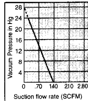
Flow Characteristics Reference Only
